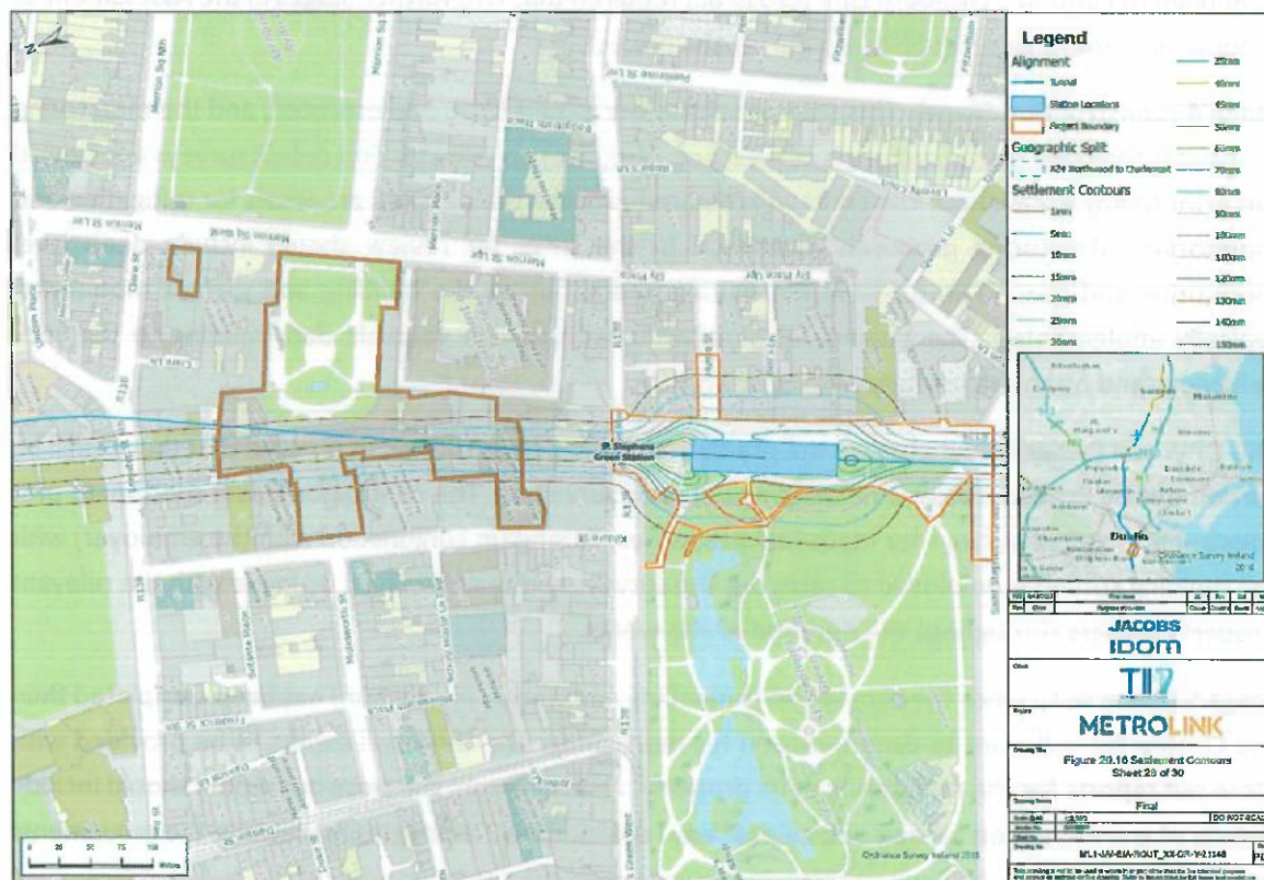
Figure 18. Settlement Contours (Extract from ML1-JAI-EIA-ROUT_XX-DR-Y-21148)
