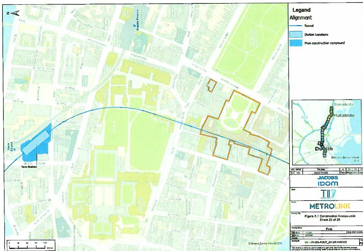
Figure 16. Plan Showing Horizontal Alignment (extract from ML1-JAI-EIA-ROUT_XX-DR-Y-05025)
